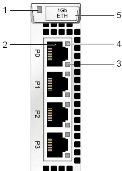
Figure 4-8 GE electrical interface module
