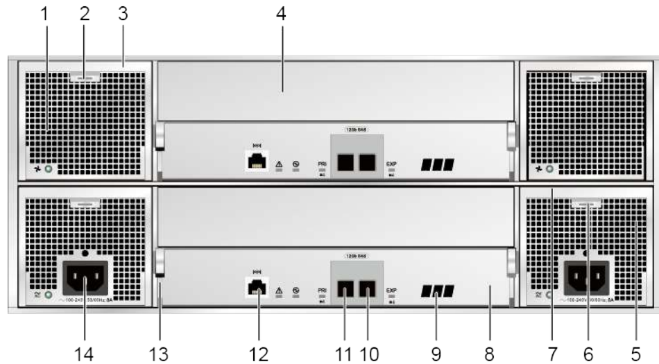
Figure 4-22 Rear view of a disk enclosure
