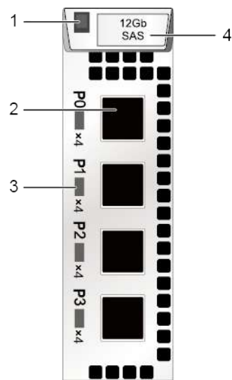
Figure 4-13 12 Gbit/s SAS expansion module
