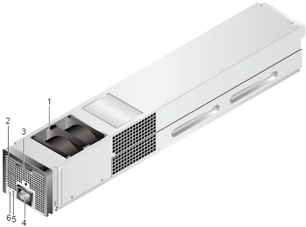
Figure 4-14 Front view of an AC power-BBU module
